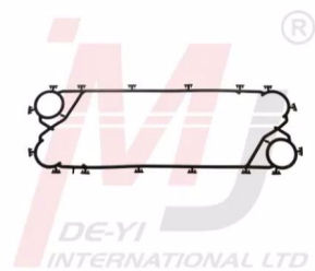
1255600 Caterpillar 3406E/3412E/C15/C30/C32
